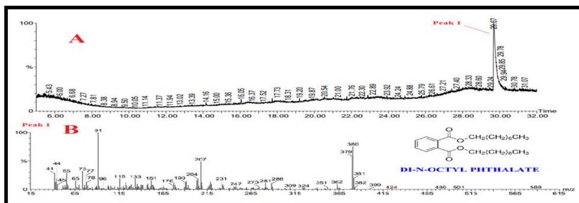
Figure 4.17: VOCs determined using GC/MS in extract of Streptomyces cellulosa DST28
